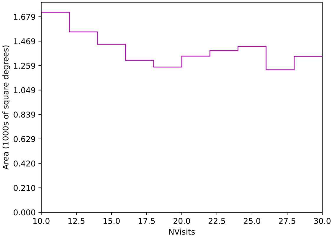
too_elab_r16_d3_giz_v3.4_10yrs Yr 3-4 z band: NVisits
