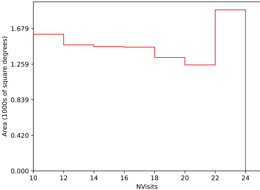
too_elab_r16_d3_giz_v3.4_10yrs Yr 3-4 i band: NVisits
