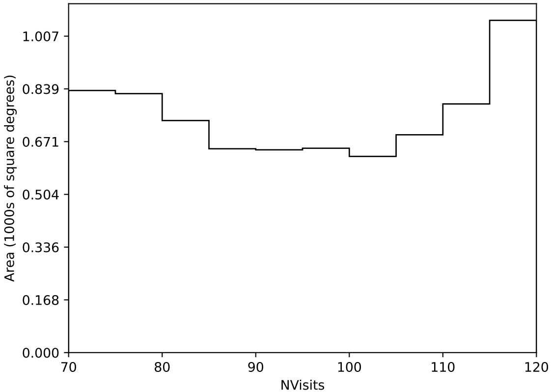
too_elab_r16_d3_giz_v3.4_10yrs Yr 3-4 all bands: NVisits
