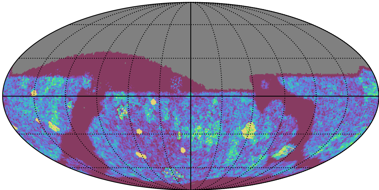
too_elab_r16_d3_giz_v3.4_10yrs Yr 1 z band: NVisits
