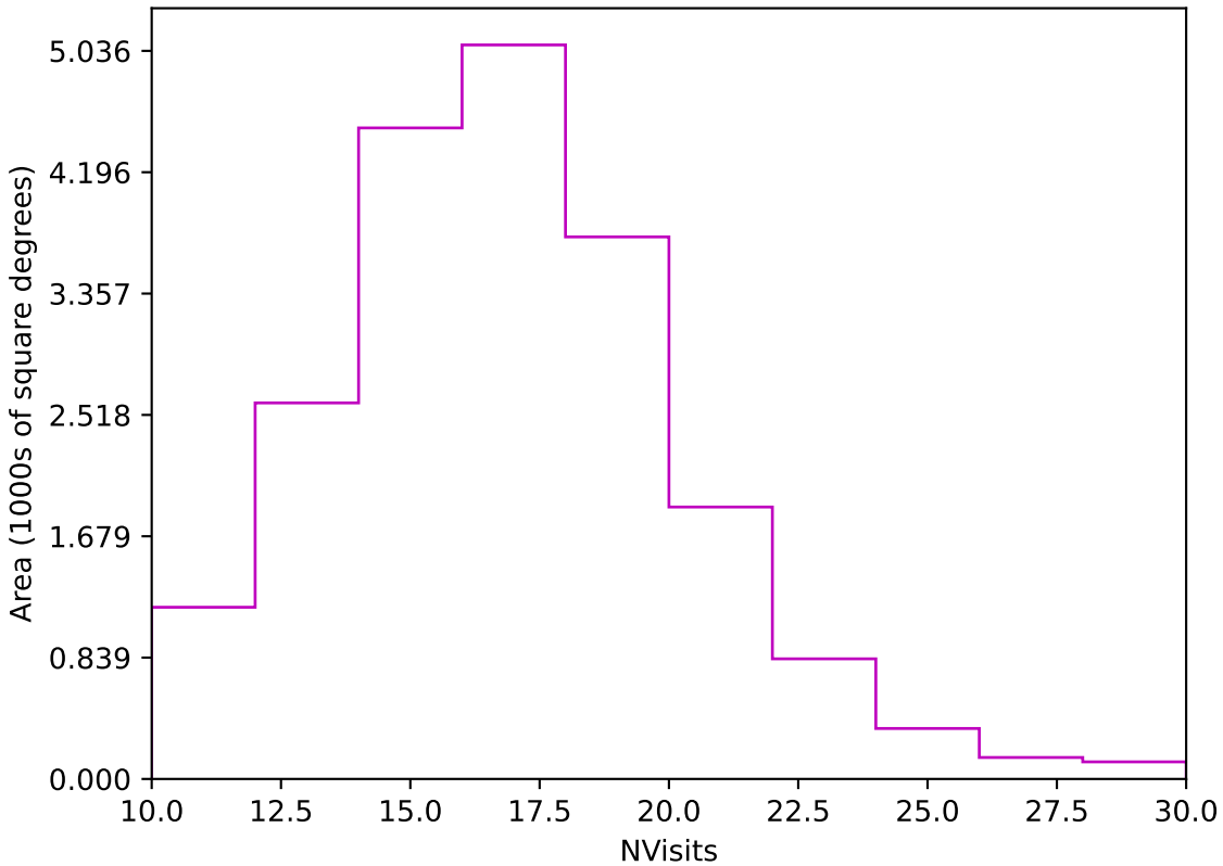
too_elab_r16_d3_giz_v3.4_10yrs Yr 1 z band: NVisits
