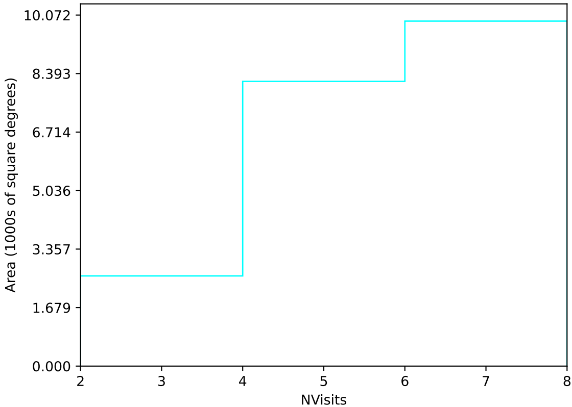
too_elab_r16_d3_giz_v3.4_10yrs Yr 1 u band: NVisits
