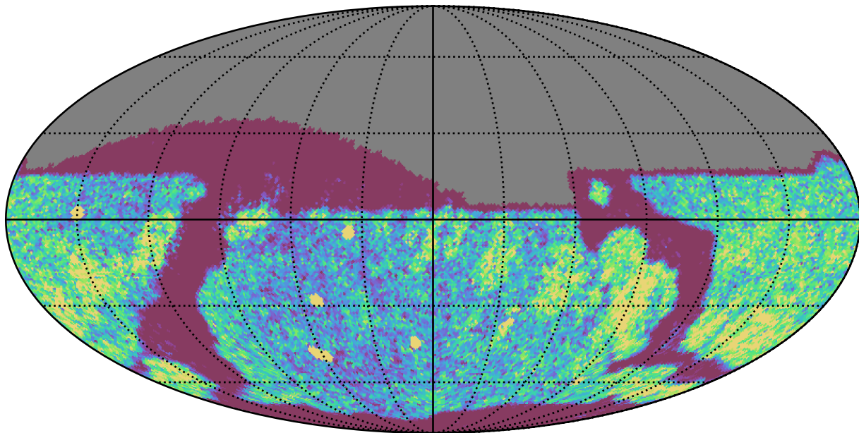
too_elab_r16_d3_giz_v3.4_10yrs Yr 1 r band: NVisits
