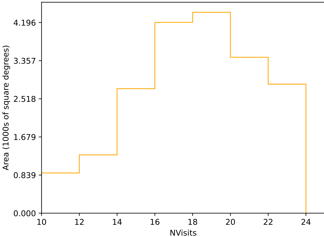
too_elab_r16_d3_giz_v3.4_10yrs Yr 1 r band: NVisits
