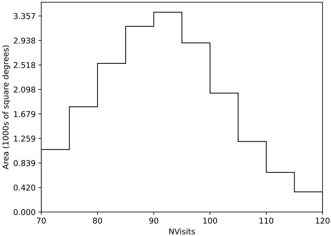
too_elab_r16_d3_giz_v3.4_10yrs Yr 1 all bands: NVisits
