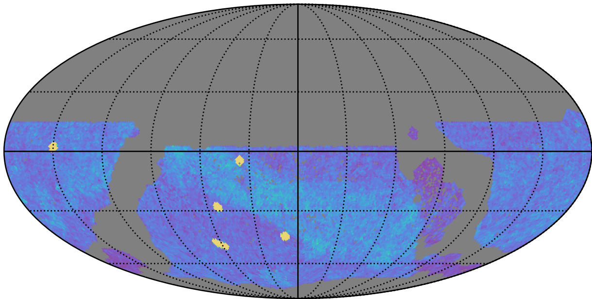
too_elab_r16_d3_giz_v3.4_10yrs WFD z band: NVisits
