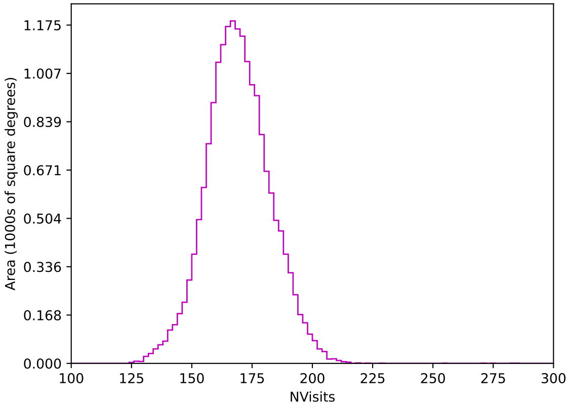
too_elab_r16_d3_giz_v3.4_10yrs WFD z band: NVisits
