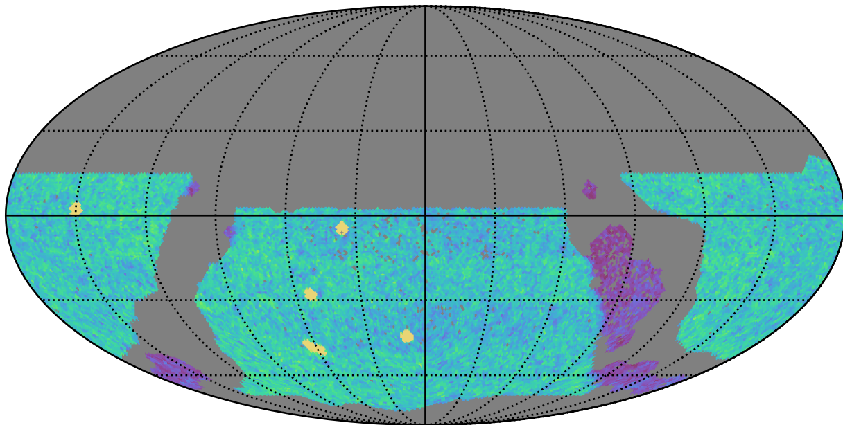
too_elab_r16_d3_giz_v3.4_10yrs WFD u band: NVisits
