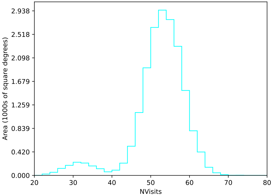
too_elab_r16_d3_giz_v3.4_10yrs WFD u band: NVisits
