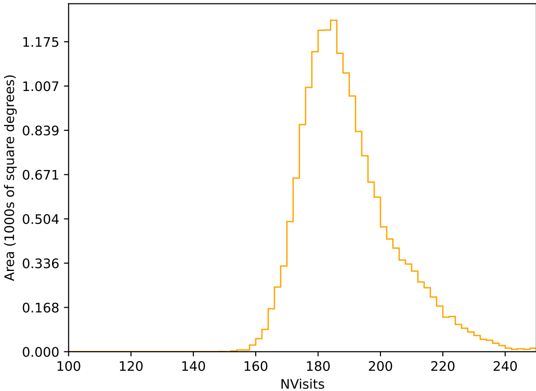
too_elab_r16_d3_giz_v3.4_10yrs WFD r band: NVisits
