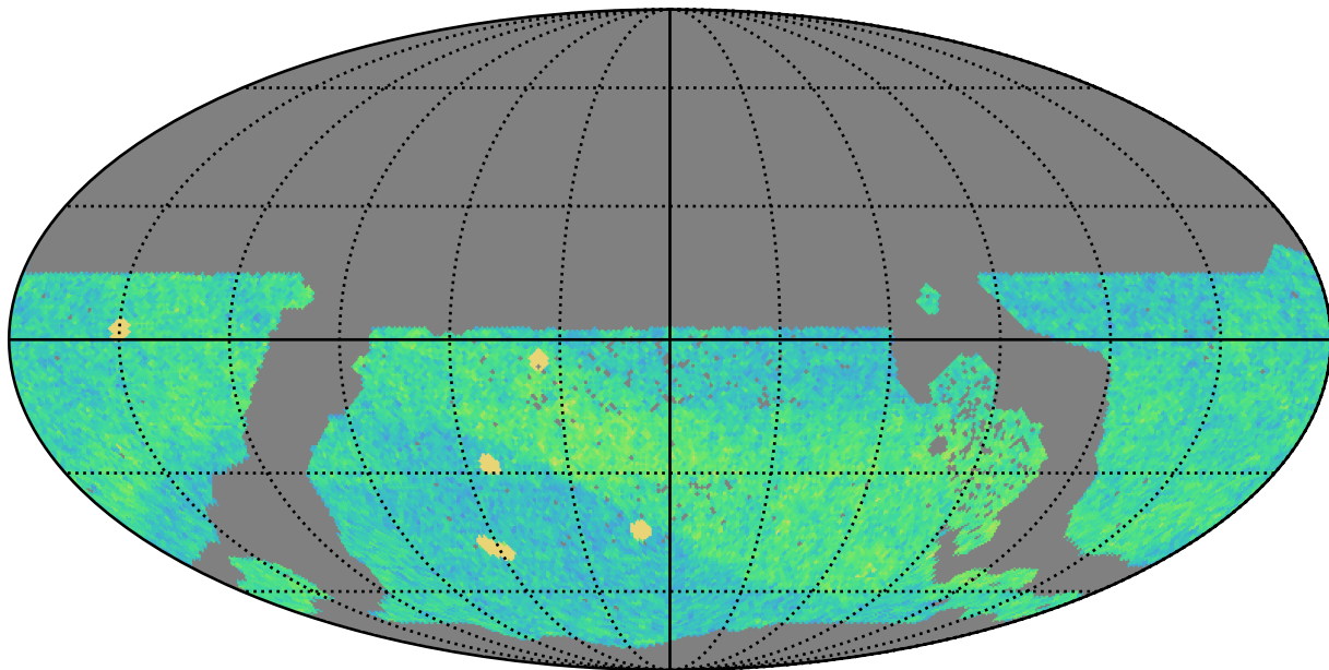
too_elab_r16_d3_giz_v3.4_10yrs WFD i band: NVisits
