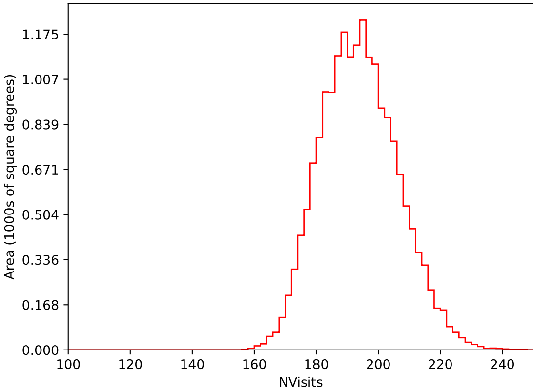
too_elab_r16_d3_giz_v3.4_10yrs WFD i band: NVisits
