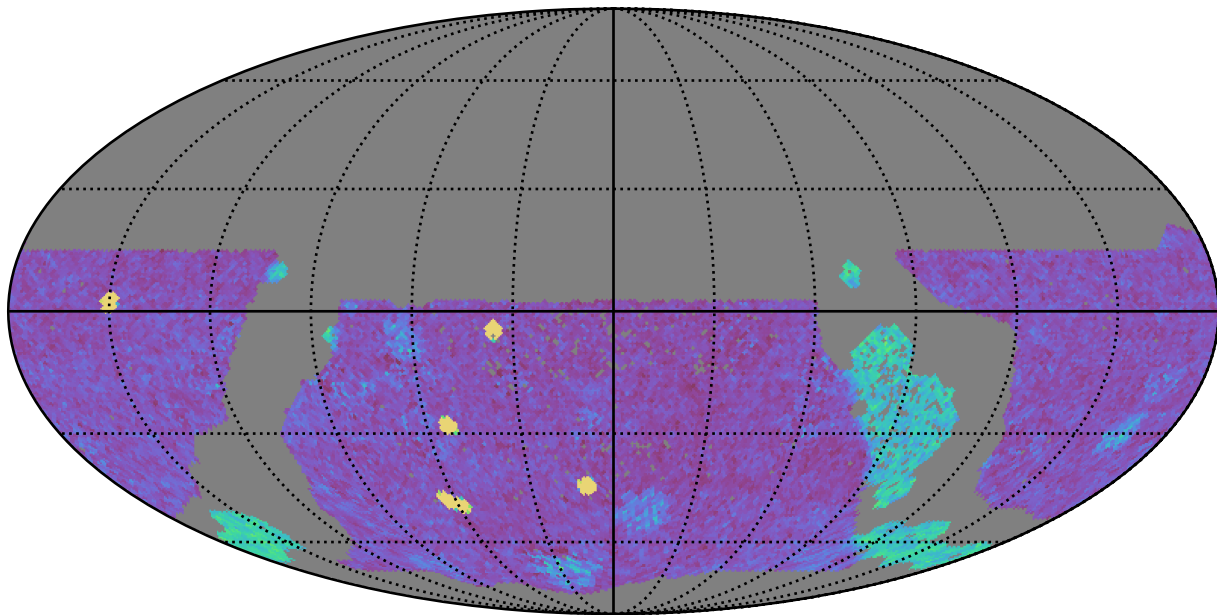
too_elab_r16_d3_giz_v3.4_10yrs WFD g band: NVisits
