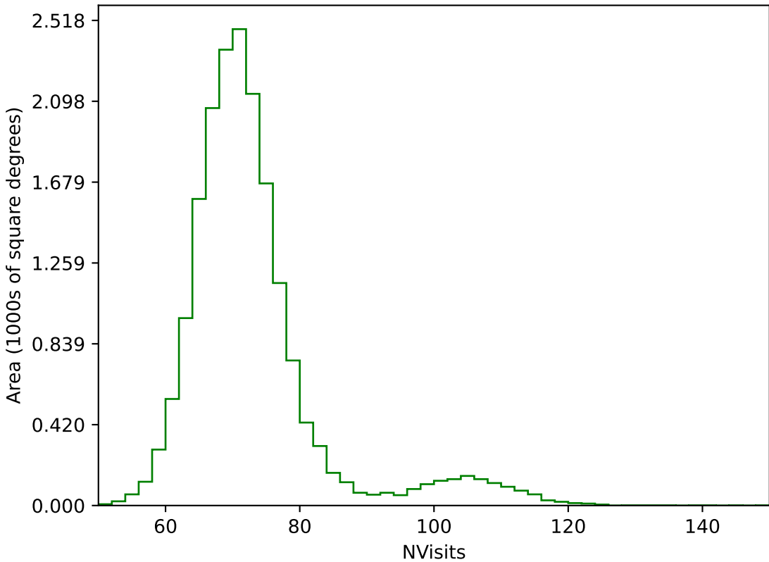
too_elab_r16_d3_giz_v3.4_10yrs WFD g band: NVisits
