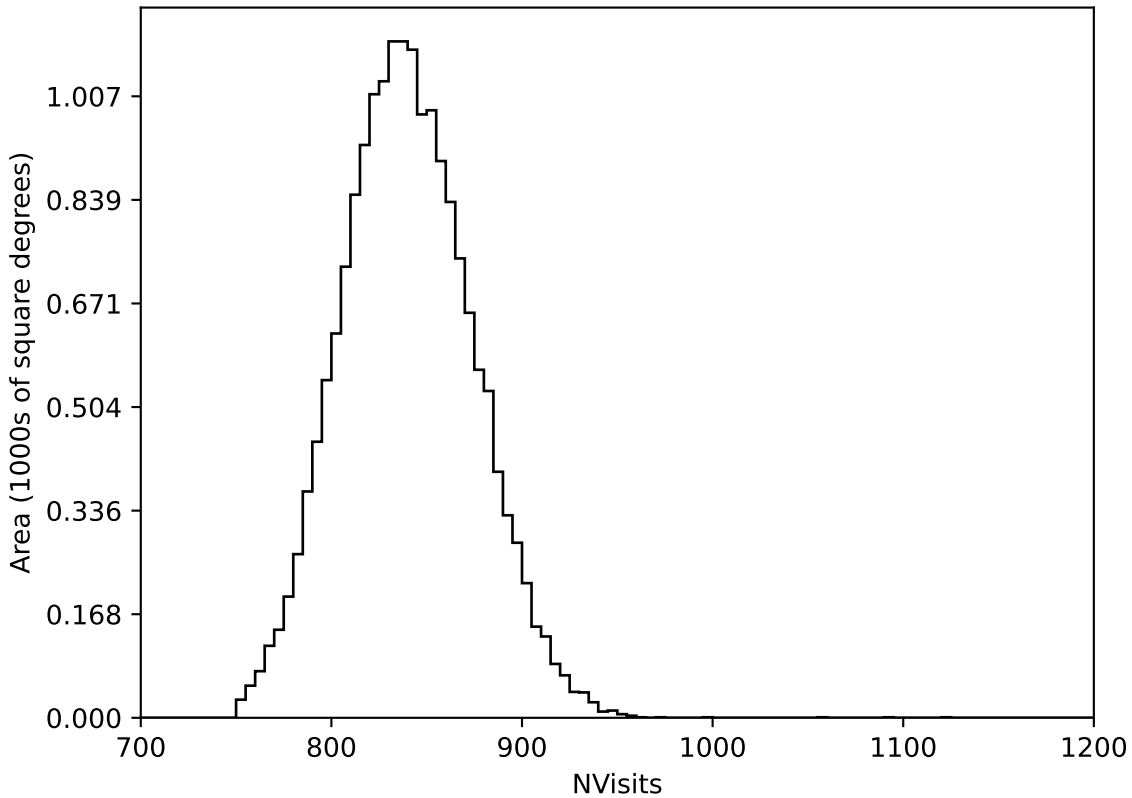
too_elab_r16_d3_giz_v3.4_10yrs WFD all bands: NVisits
