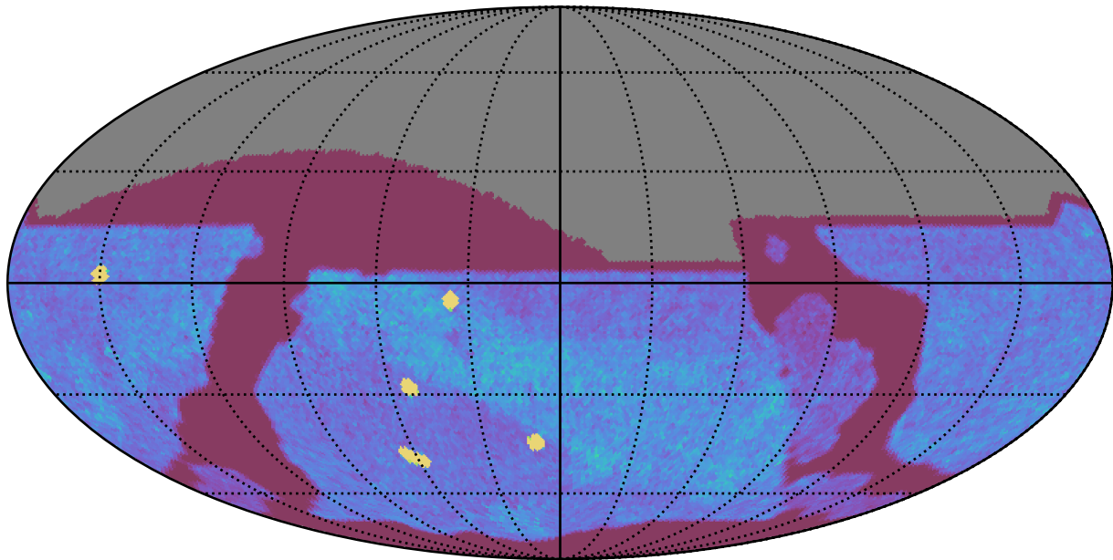
too_elab_r16_d3_giz_v3.4_10yrs All sky z band: NVisits
