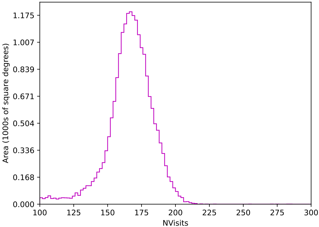
too_elab_r16_d3_giz_v3.4_10yrs All sky z band: NVisits
