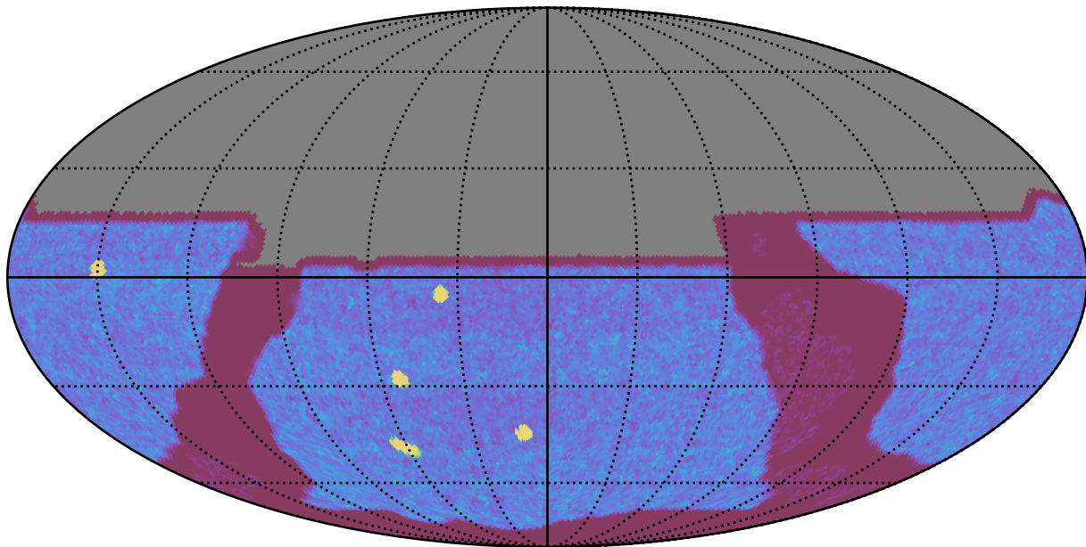
too_elab_r16_d3_giz_v3.4_10yrs All sky y band: NVisits
