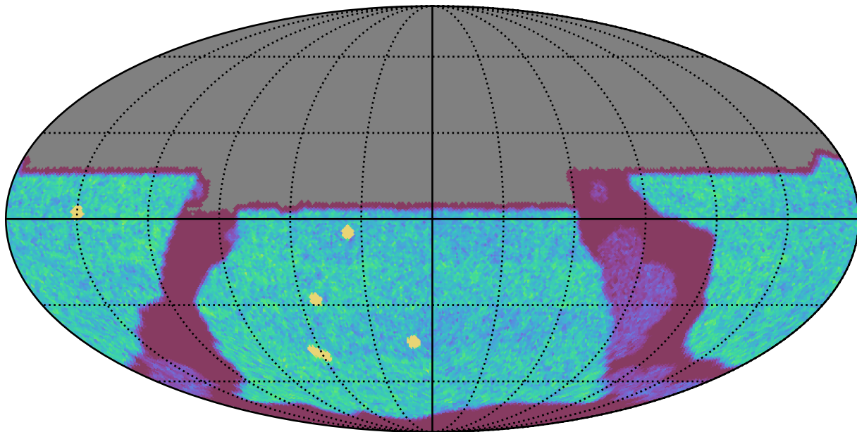
too_elab_r16_d3_giz_v3.4_10yrs All sky u band: NVisits
