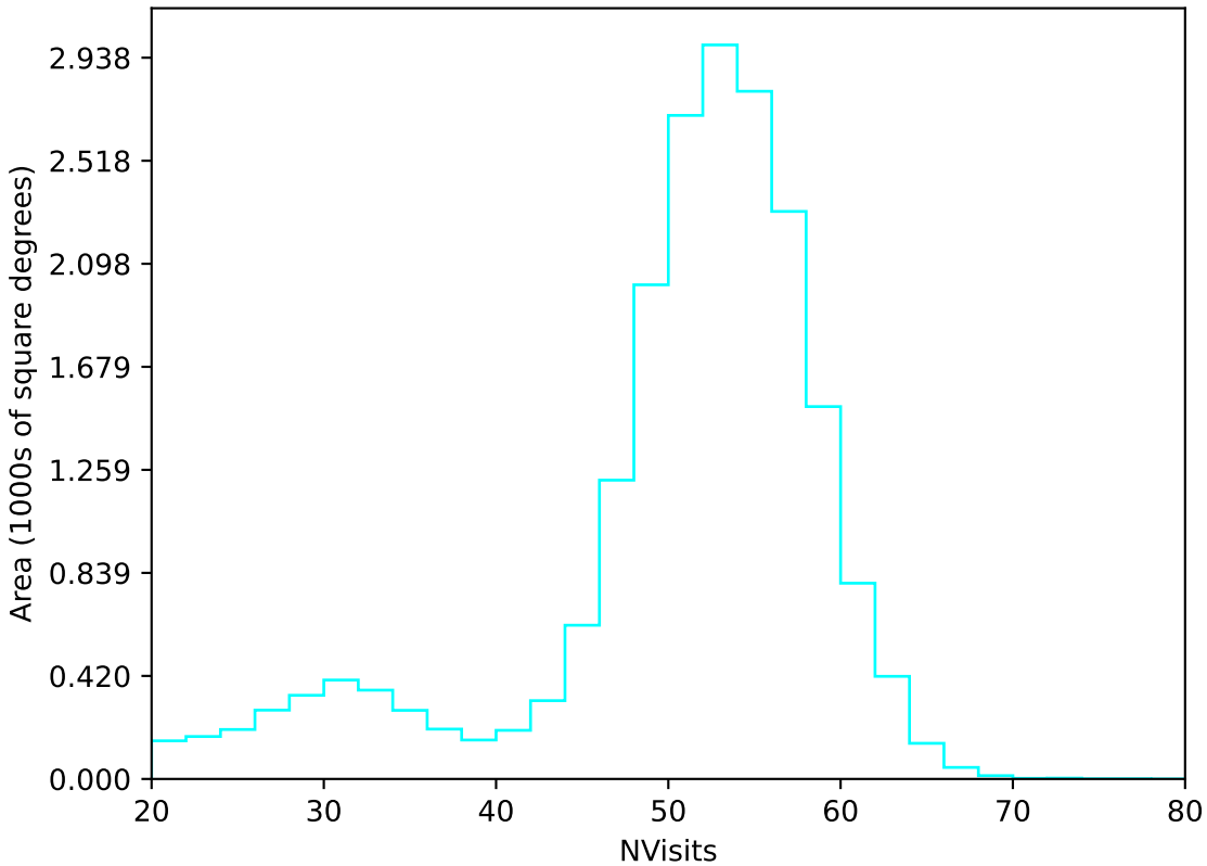
too_elab_r16_d3_giz_v3.4_10yrs All sky u band: NVisits
