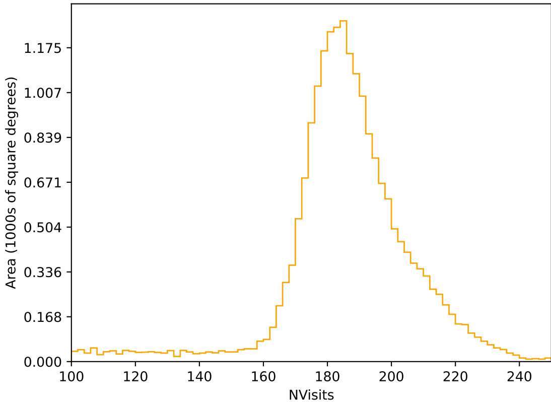
too_elab_r16_d3_giz_v3.4_10yrs All sky r band: NVisits
