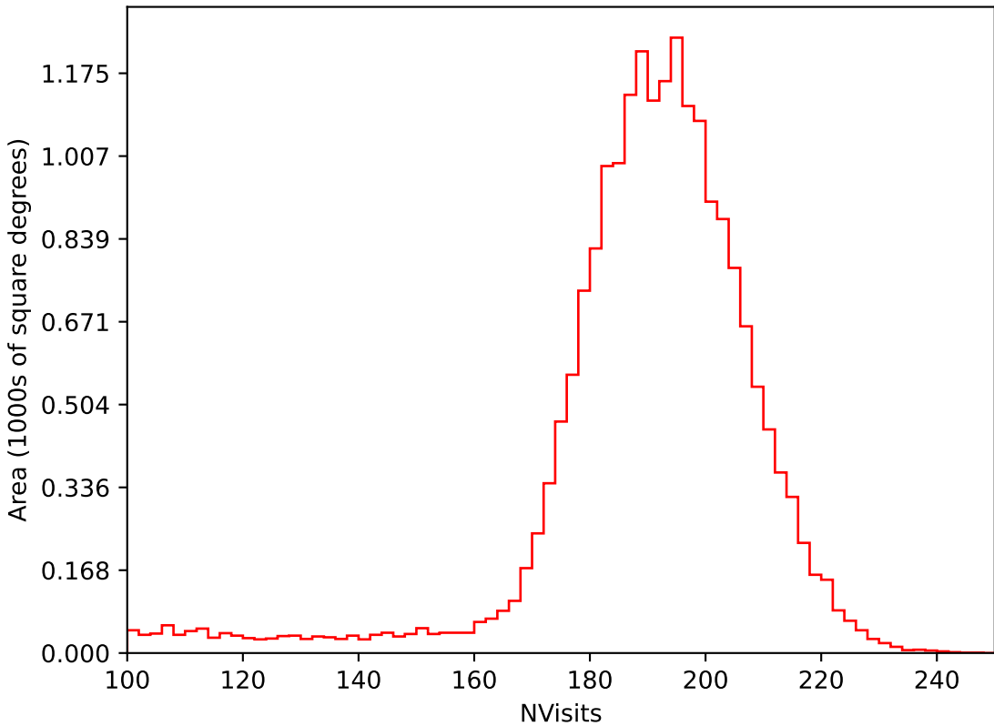
too_elab_r16_d3_giz_v3.4_10yrs All sky i band: NVisits
