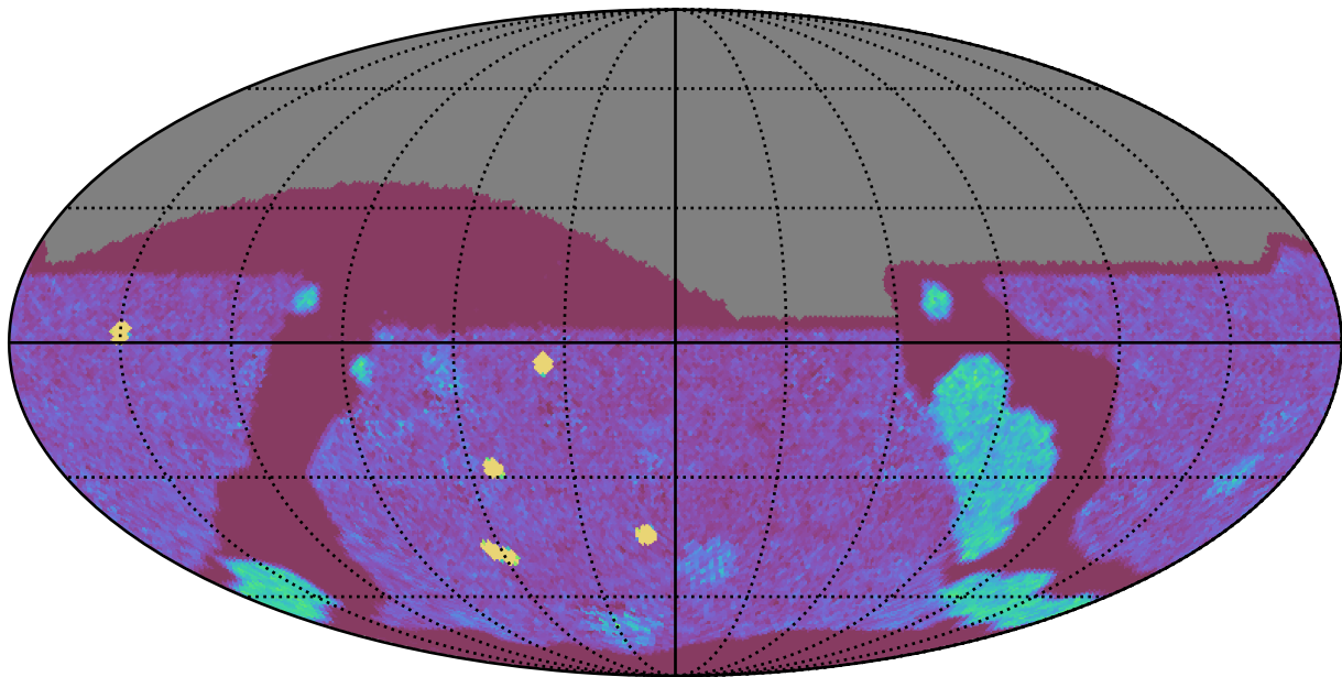
too_elab_r16_d3_giz_v3.4_10yrs All sky g band: NVisits
