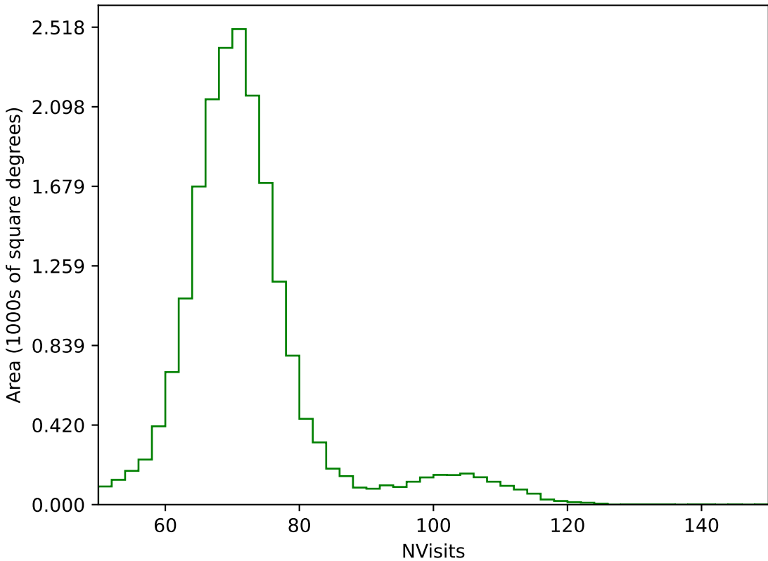
too_elab_r16_d3_giz_v3.4_10yrs All sky g band: NVisits
