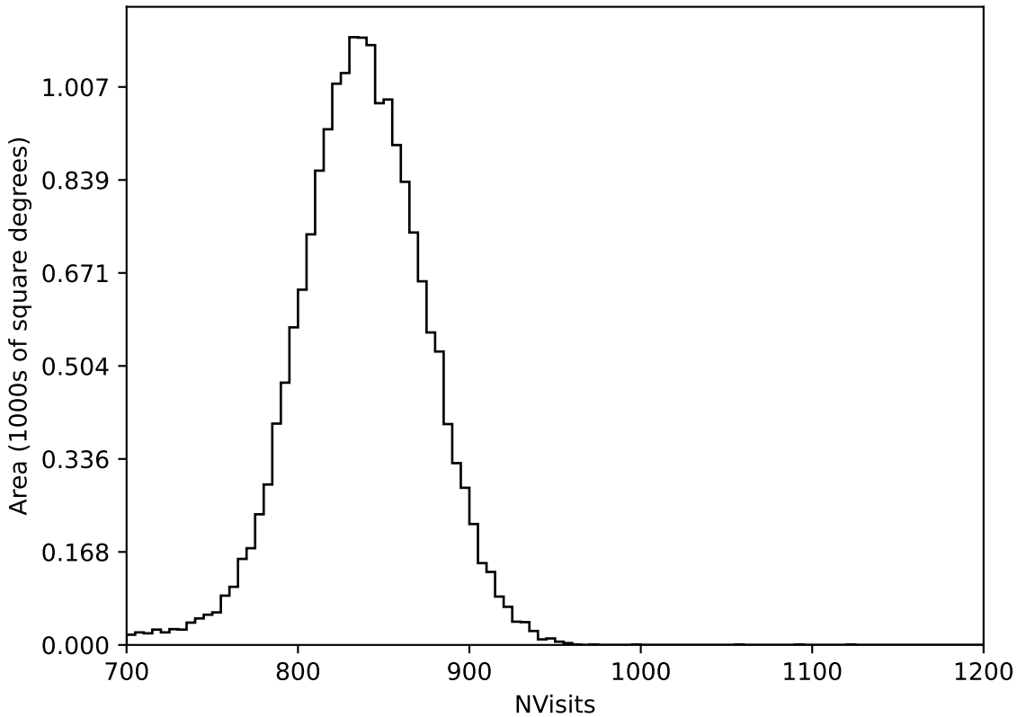
too_elab_r16_d3_giz_v3.4_10yrs All sky all bands: NVisits
