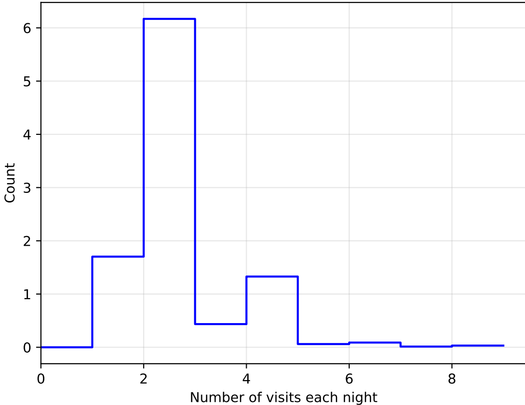
too_elab_r16_d3_giz_v3.4_10yrs All sky: NVisitsPerNight
