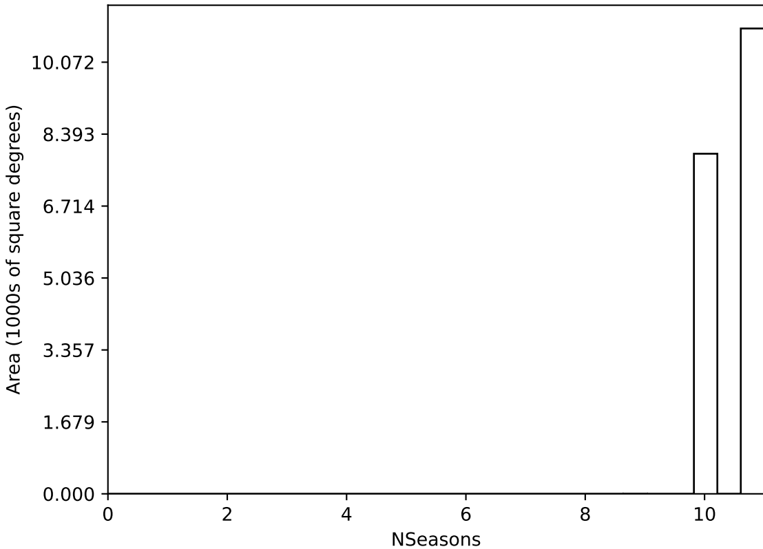
too_elab_r16_d3_giz_v3.4_10yrs WFD all bands: NSeasons
