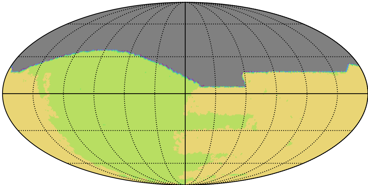
too_elab_r16_d3_giz_v3.4_10yrs All sky all bands: NSeasons
