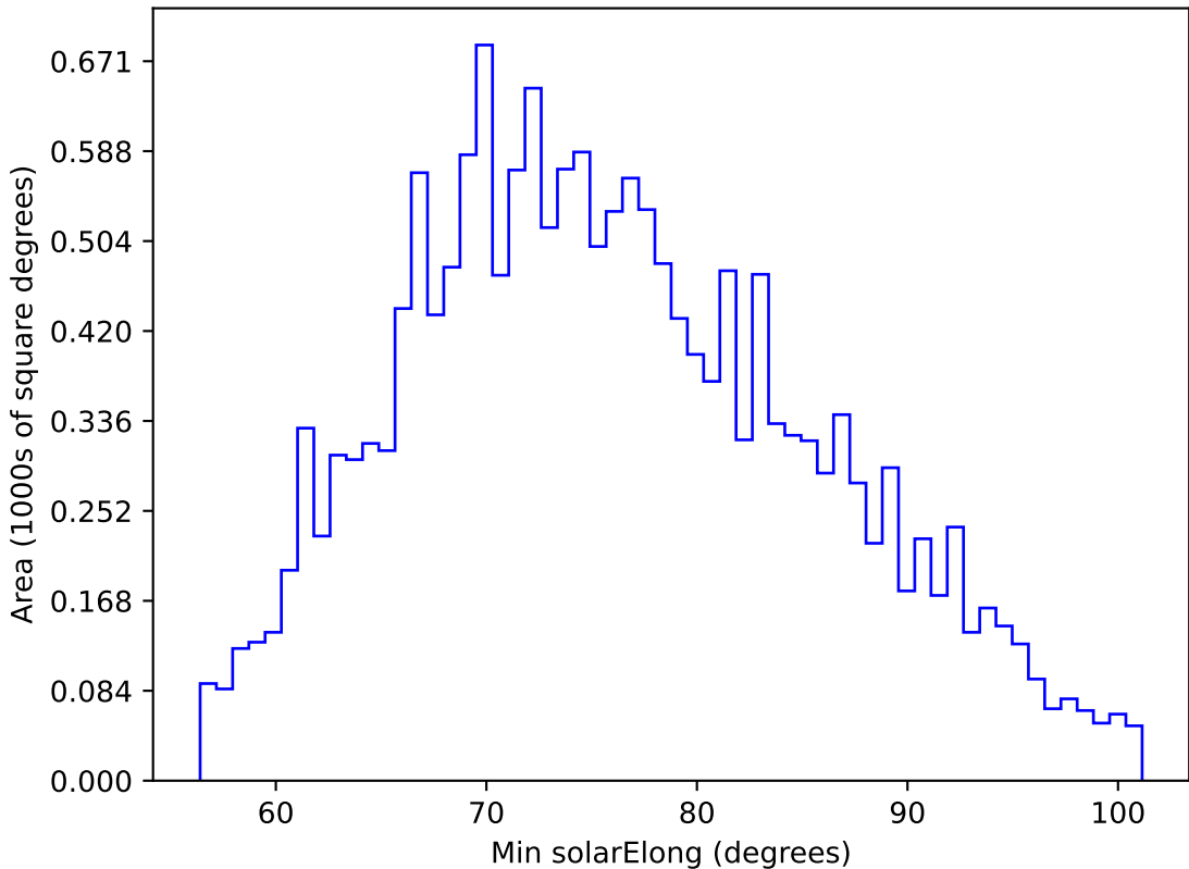
too_elab_r16_d3_giz_v3.4_10yrs WFD u band: Min solarElong
