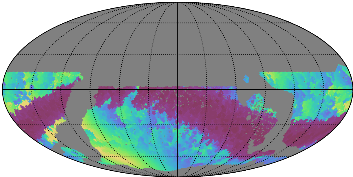
too_elab_r16_d3_giz_v3.4_10yrs WFD r band: Min solarElong
