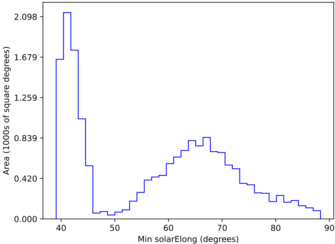
too_elab_r16_d3_giz_v3.4_10yrs WFD r band: Min solarElong
