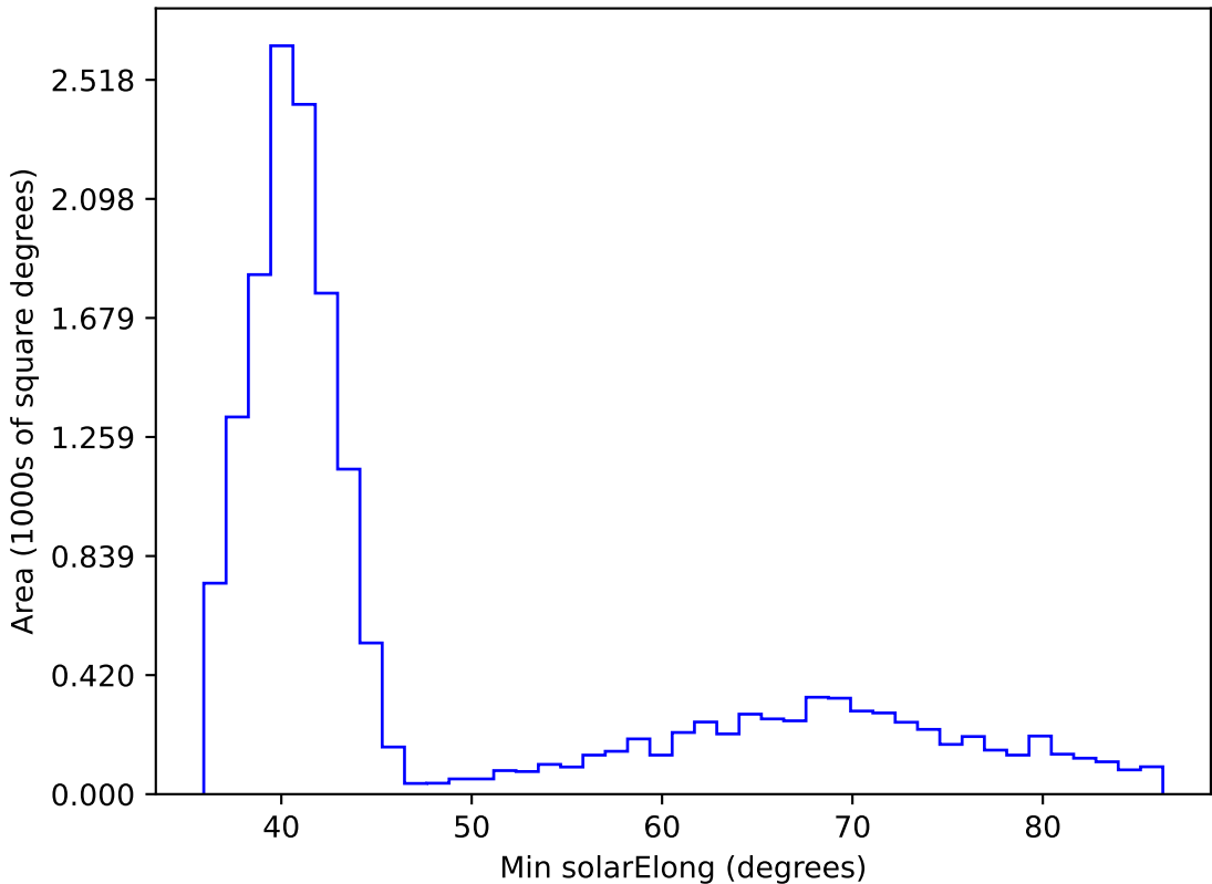
too_elab_r16_d3_giz_v3.4_10yrs WFD i band: Min solarElong
