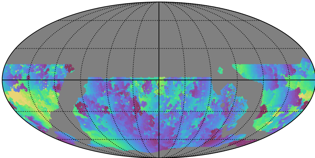
too_elab_r16_d3_giz_v3.4_10yrs WFD g band: Min solarElong
