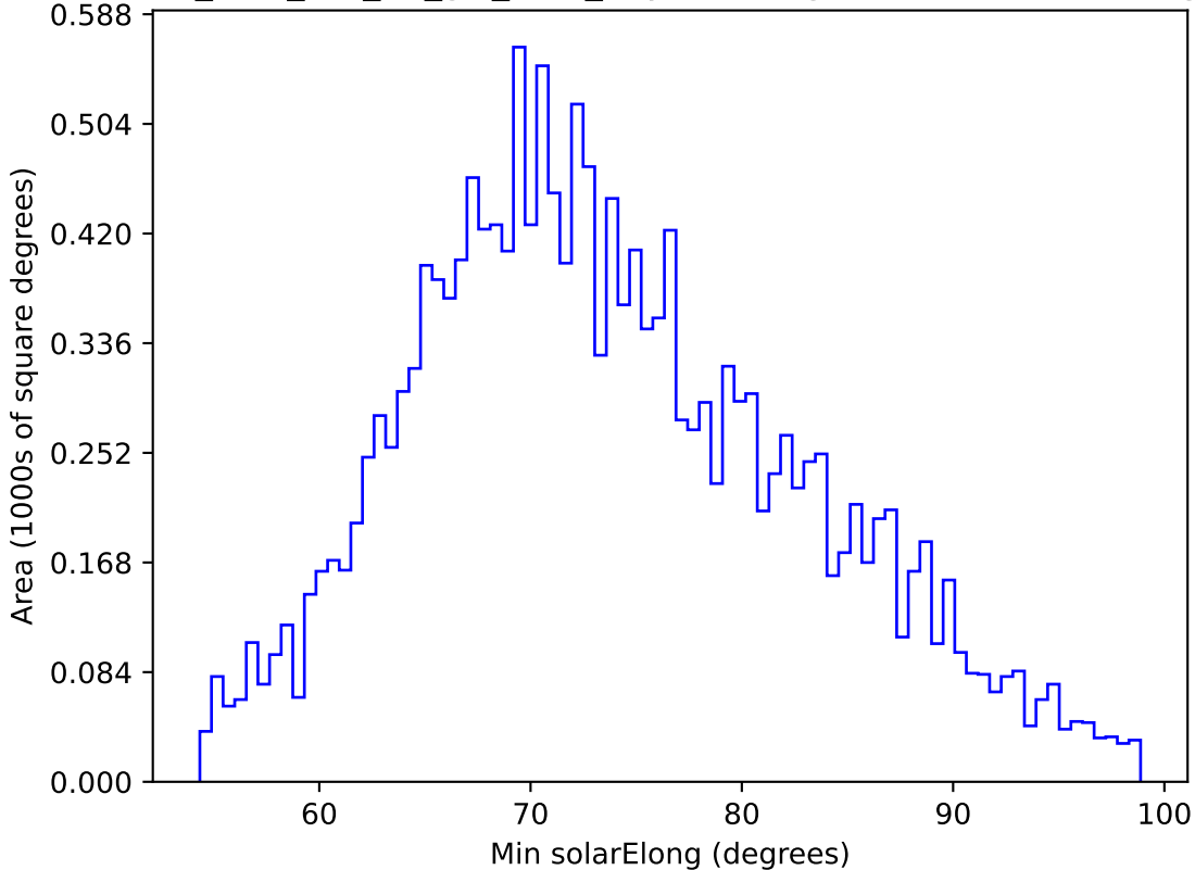
too_elab_r16_d3_giz_v3.4_10yrs WFD g band: Min solarElong
