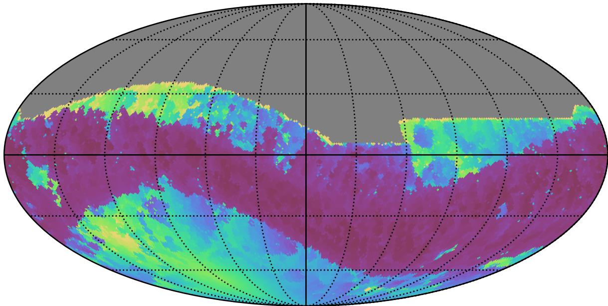
too_elab_r16_d3_giz_v3.4_10yrs All sky z band: Min solarElong
