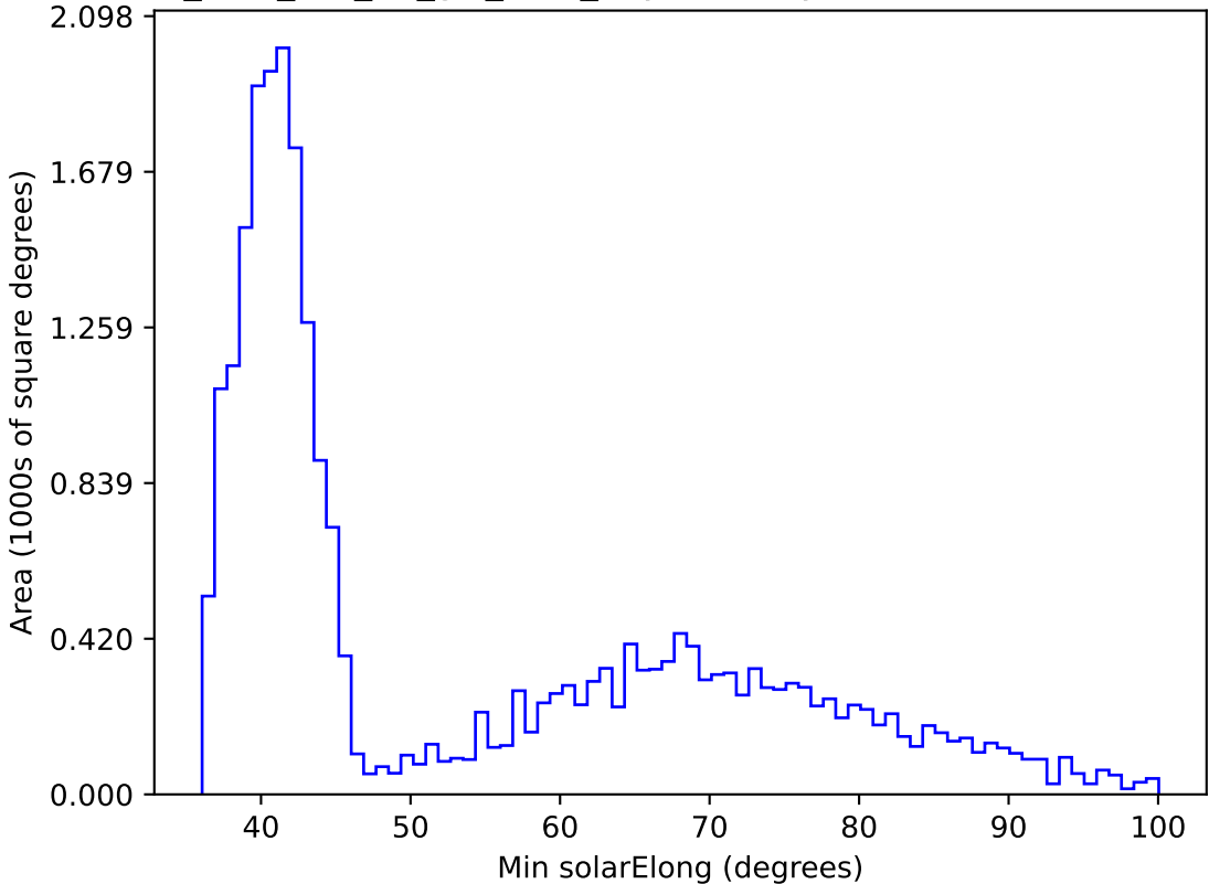
too_elab_r16_d3_giz_v3.4_10yrs All sky z band: Min solarElong
