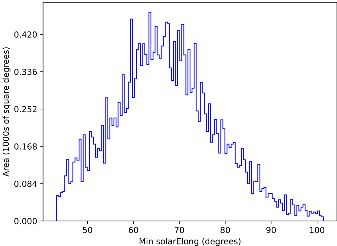
too_elab_r16_d3_giz_v3.4_10yrs All sky y band: Min solarElong
