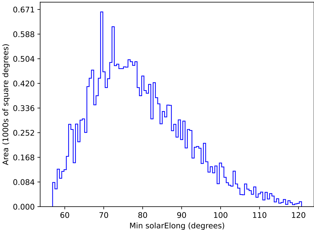
too_elab_r16_d3_giz_v3.4_10yrs All sky u band: Min solarElong
