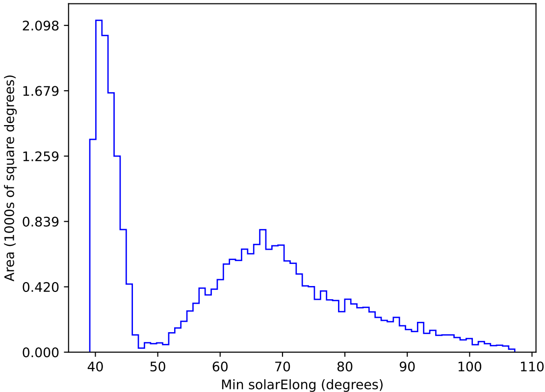
too_elab_r16_d3_giz_v3.4_10yrs All sky r band: Min solarElong
