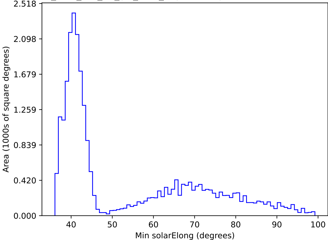
too_elab_r16_d3_giz_v3.4_10yrs All sky i band: Min solarElong
