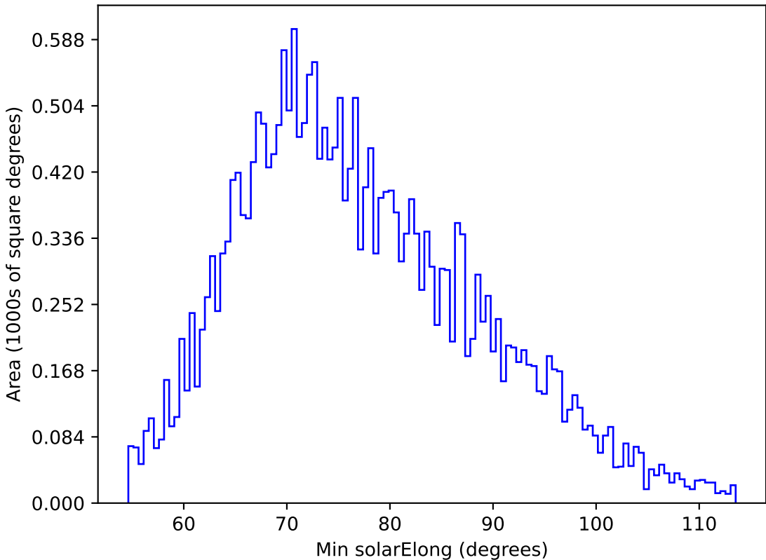
too_elab_r16_d3_giz_v3.4_10yrs All sky g band: Min solarElong
