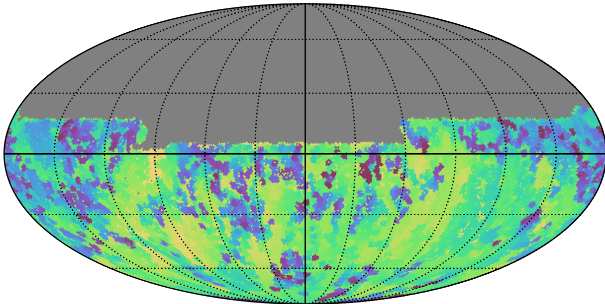
too_elab_r16_d3_giz_v3.4_10yrs Yr 1 y band: Min skyBrightness
