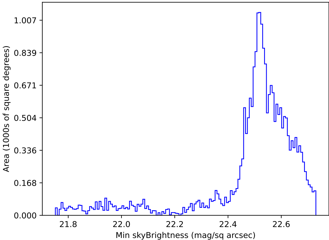
too_elab_r16_d3_giz_v3.4_10yrs Yr 1 u band: Min skyBrightness
