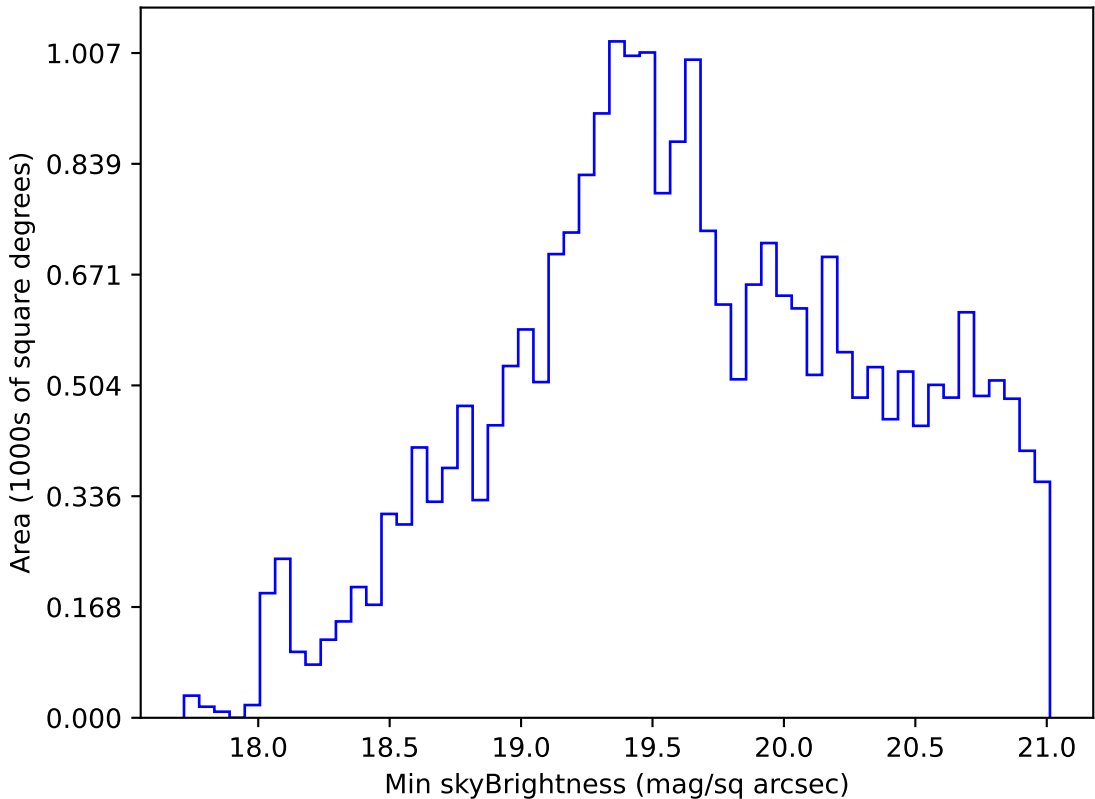
too_elab_r16_d3_giz_v3.4_10yrs Yr 1 r band: Min skyBrightness
