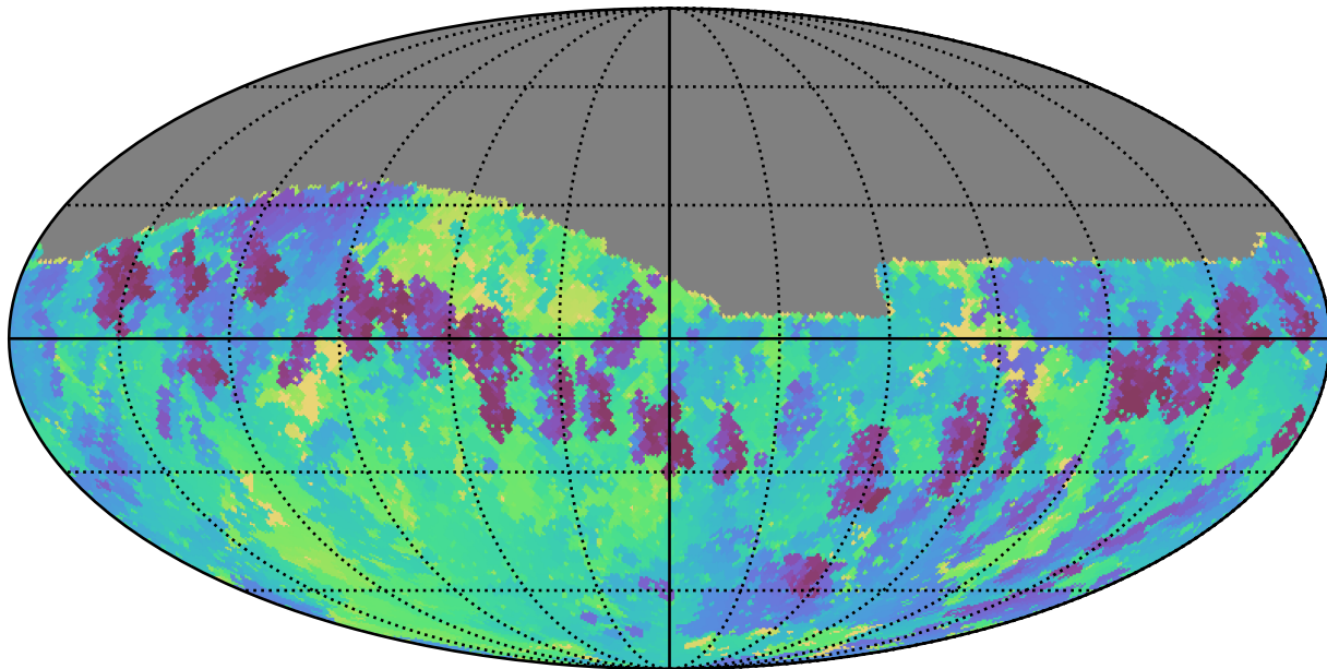
too_elab_r16_d3_giz_v3.4_10yrs Yr 1 i band: Min skyBrightness
