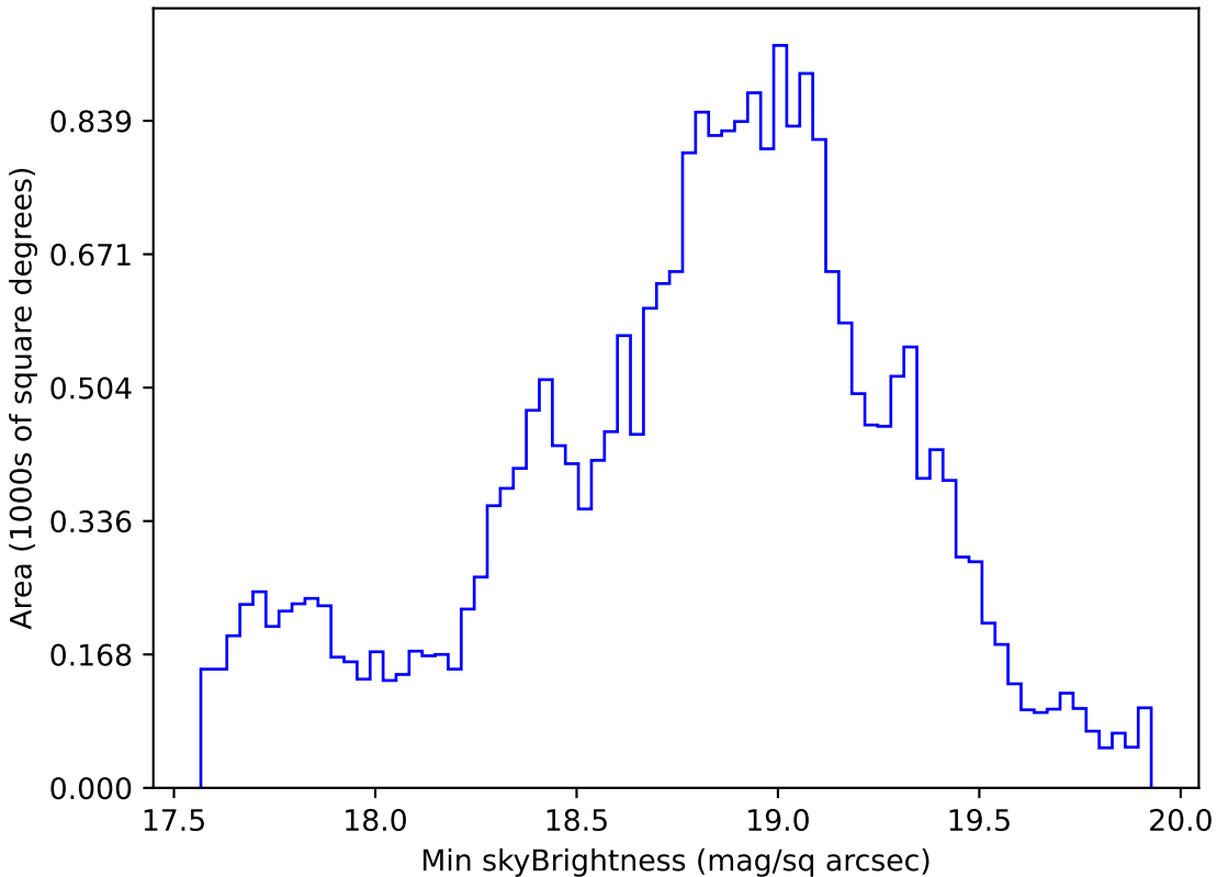
too_elab_r16_d3_giz_v3.4_10yrs Yr 1 i band: Min skyBrightness
